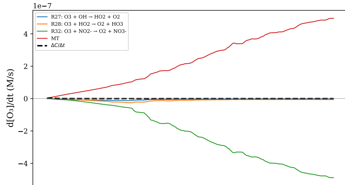
(b) \text{O}_3
