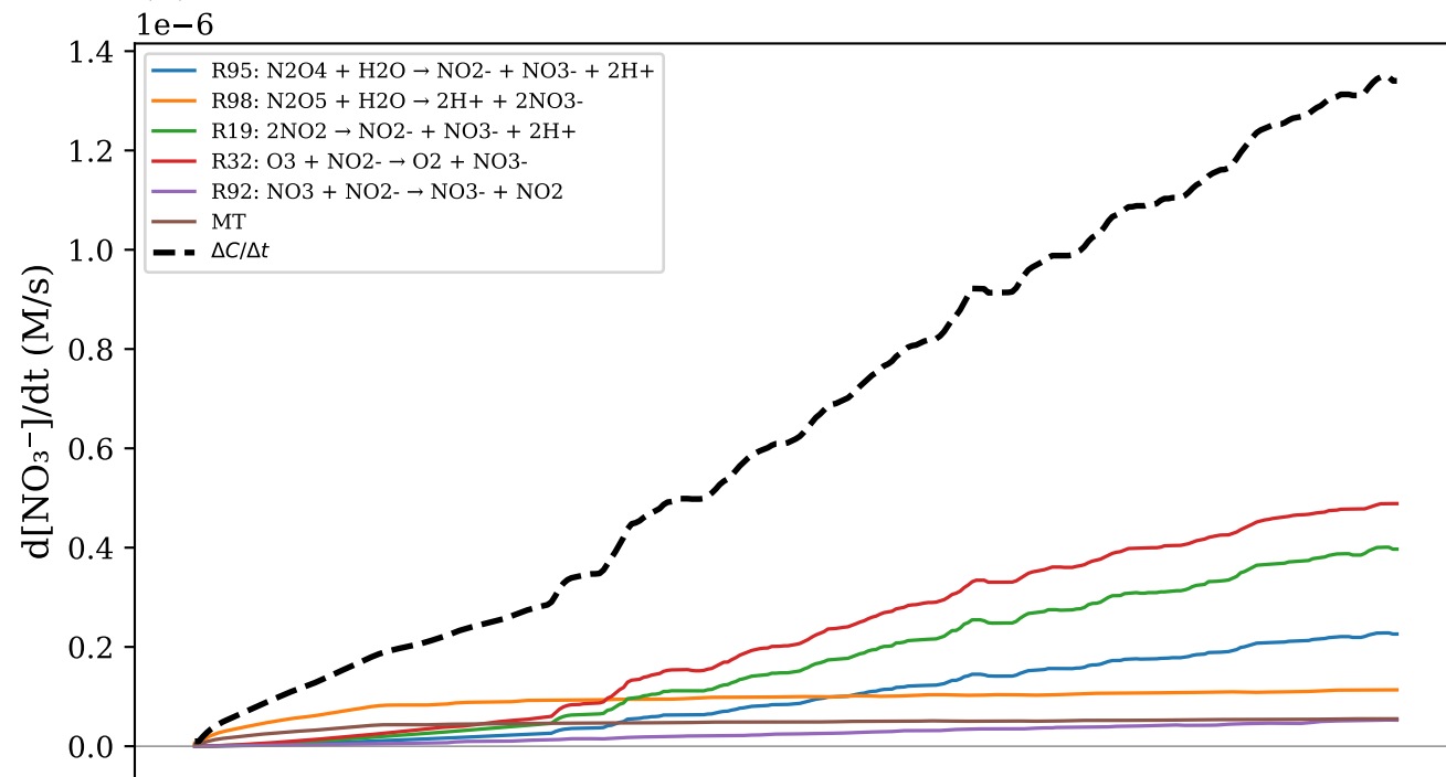
(a) \text{NO}_3^-
